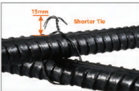
Tie height: 1.5 cm, 230 ties/coil (D23 X D23 rebar)
